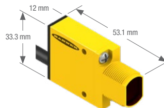
MINI-BEAM dc Suffix EPD and RPD
