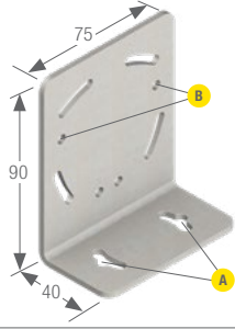
SMBLTFL (All measurements in mm)
