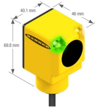
Opposed, Polarized Retroreflective and Fixed-Field Models Suffix E, R, LP and FF
