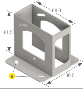
SMBLTFU (All measurements in mm)
