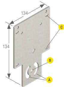
SMBAMSLTFP (All measurements in mm)
